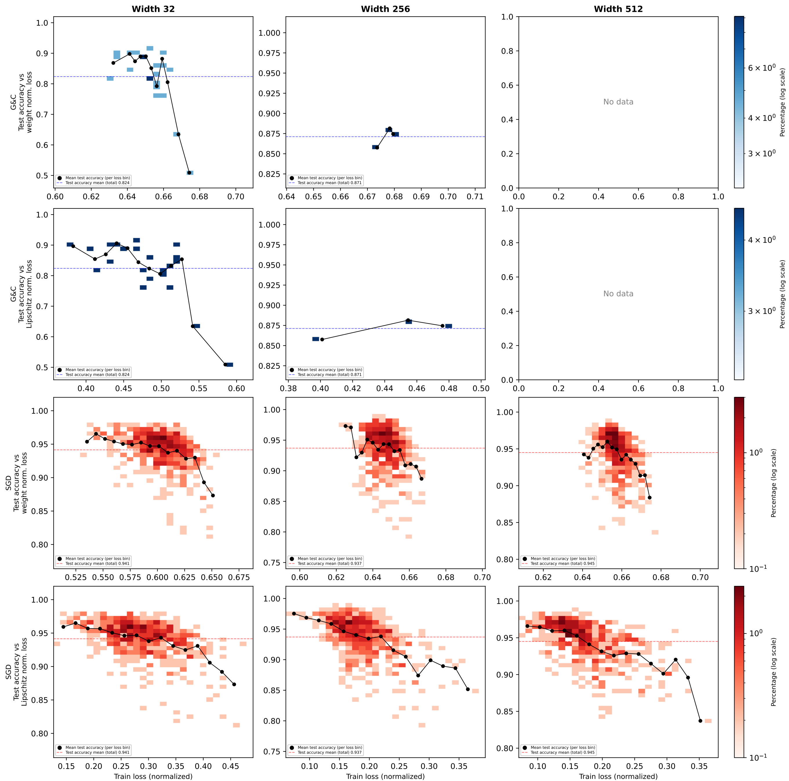
Test Accuracy vs. Normalised Train Loss — MNIST dataset Width sweep — Init: Kaiming Uniform
