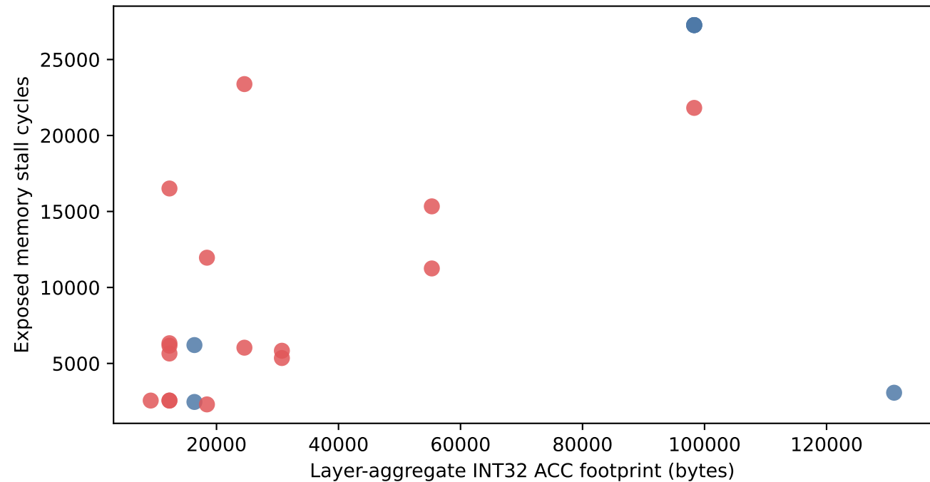
Layer-aggregate ACC footprint and exposed stall
