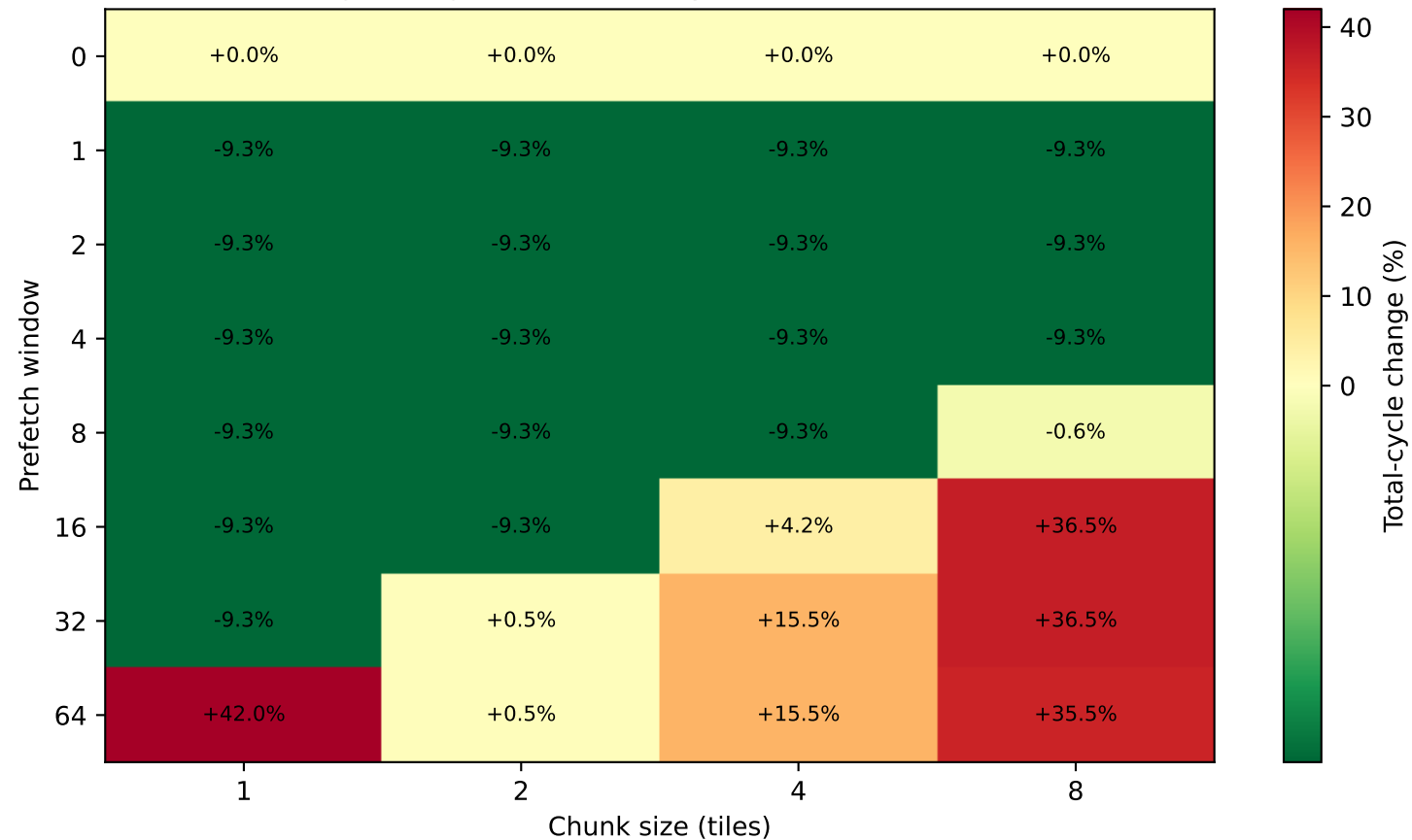
Naive prefetch total-cycle change vs NoPF (negative/green = faster; positive/red = slower)
