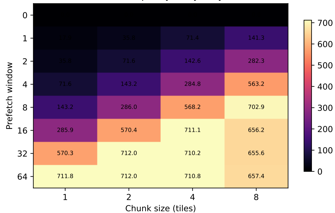
Prefetch occupancy (MByte-cycles)
