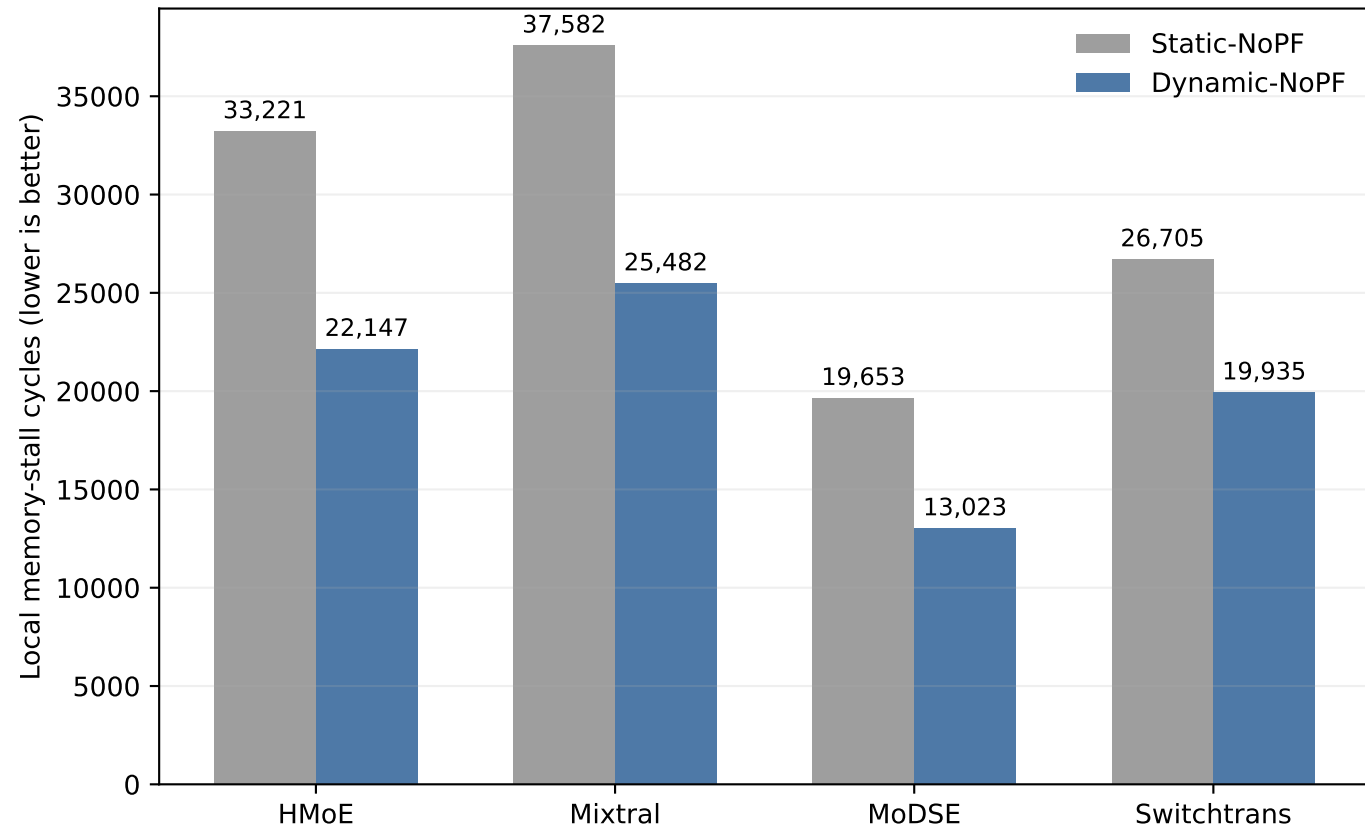
(a) Absolute local memory stall
