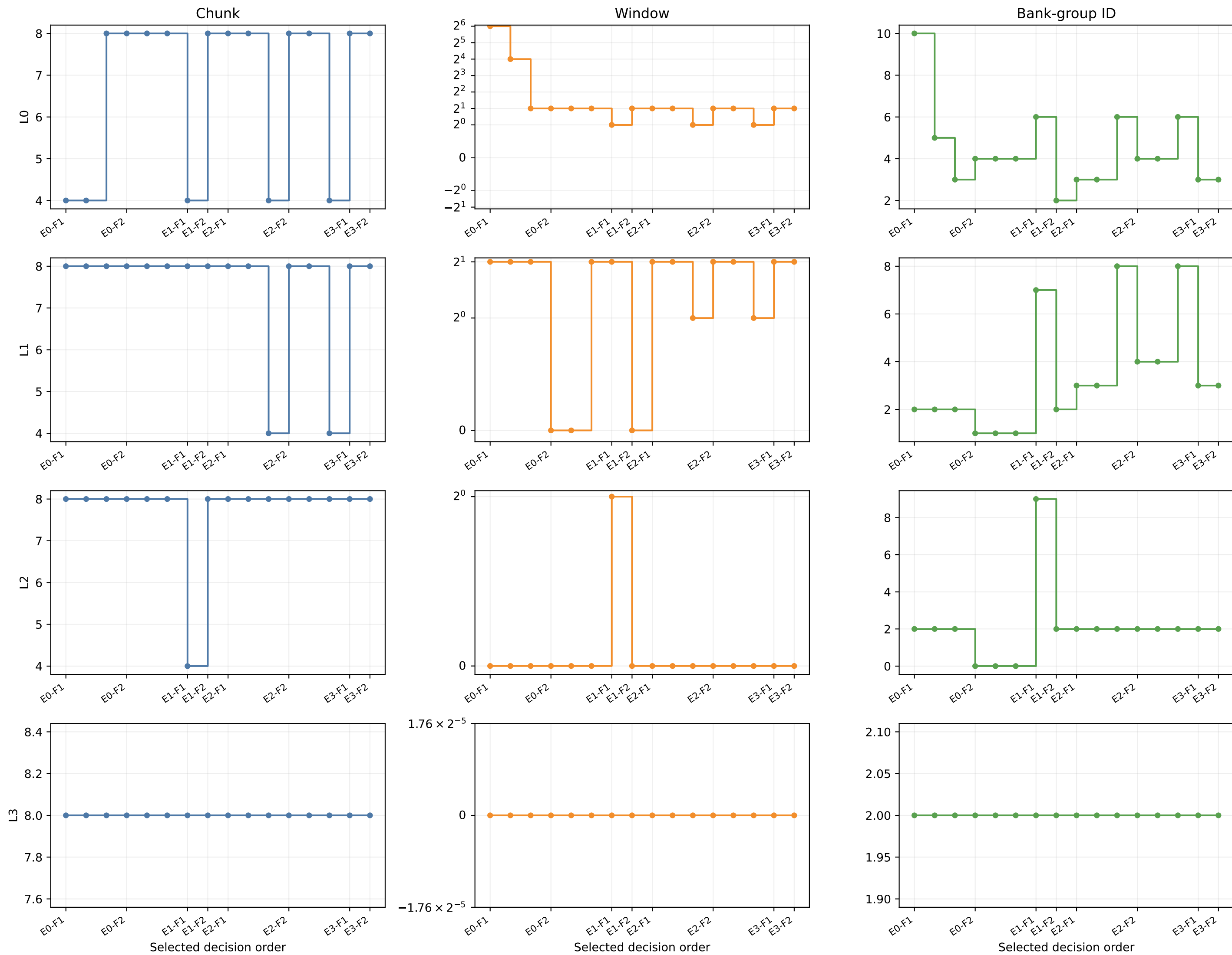
MoDSE Exp5 online decisions — every local Expert and FFN stage
