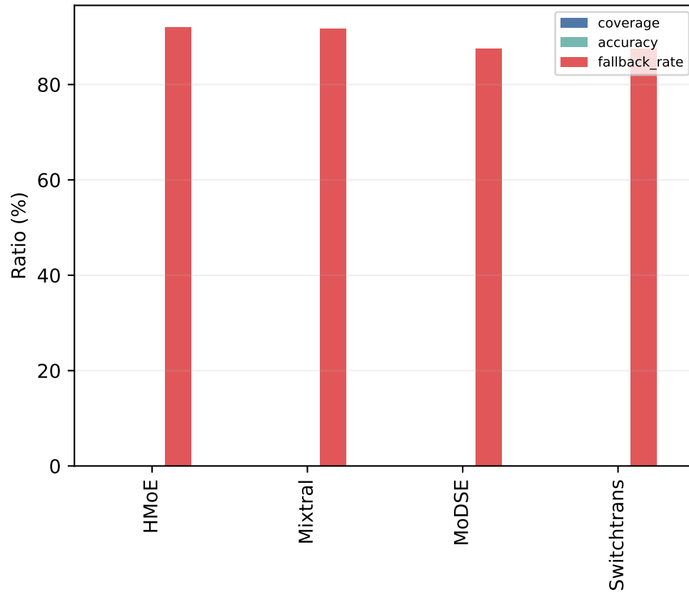
(b) Quality failure and fallback
