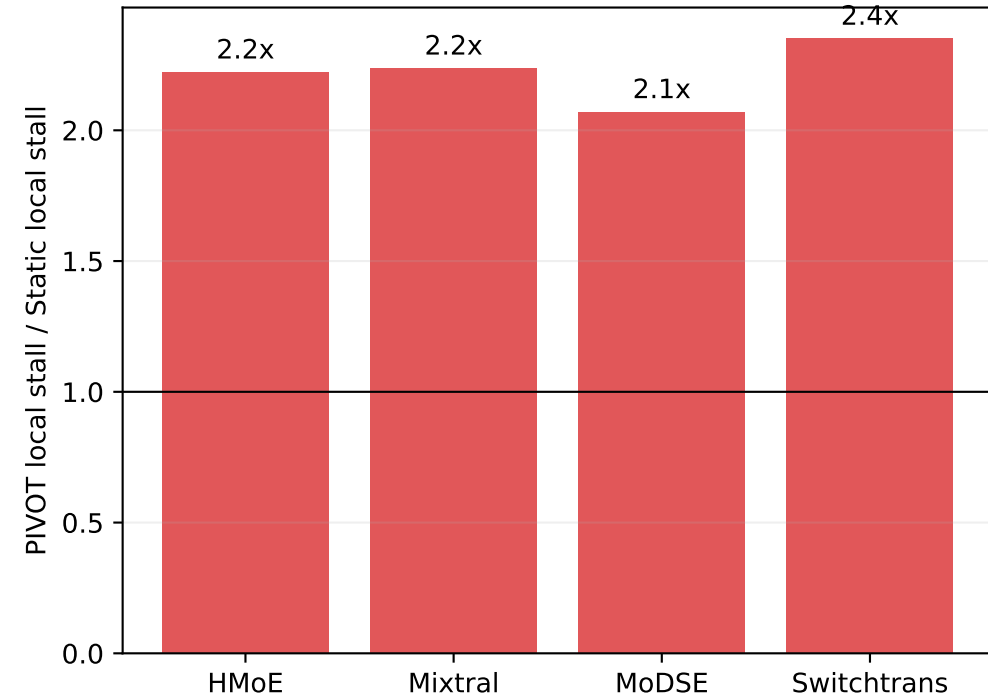
(c) Local-stall inflation
