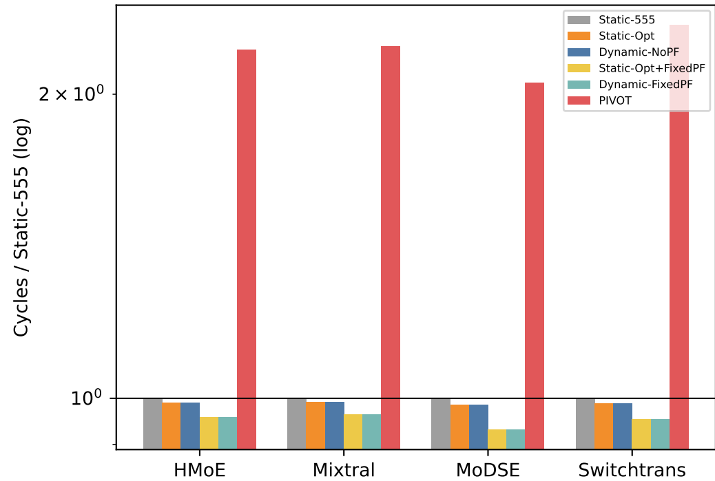
(a) Token=32 short-sequence case
