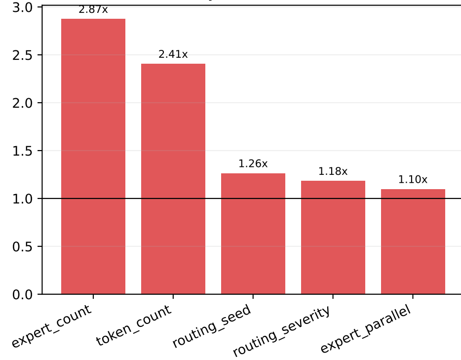
Cycle inflation
