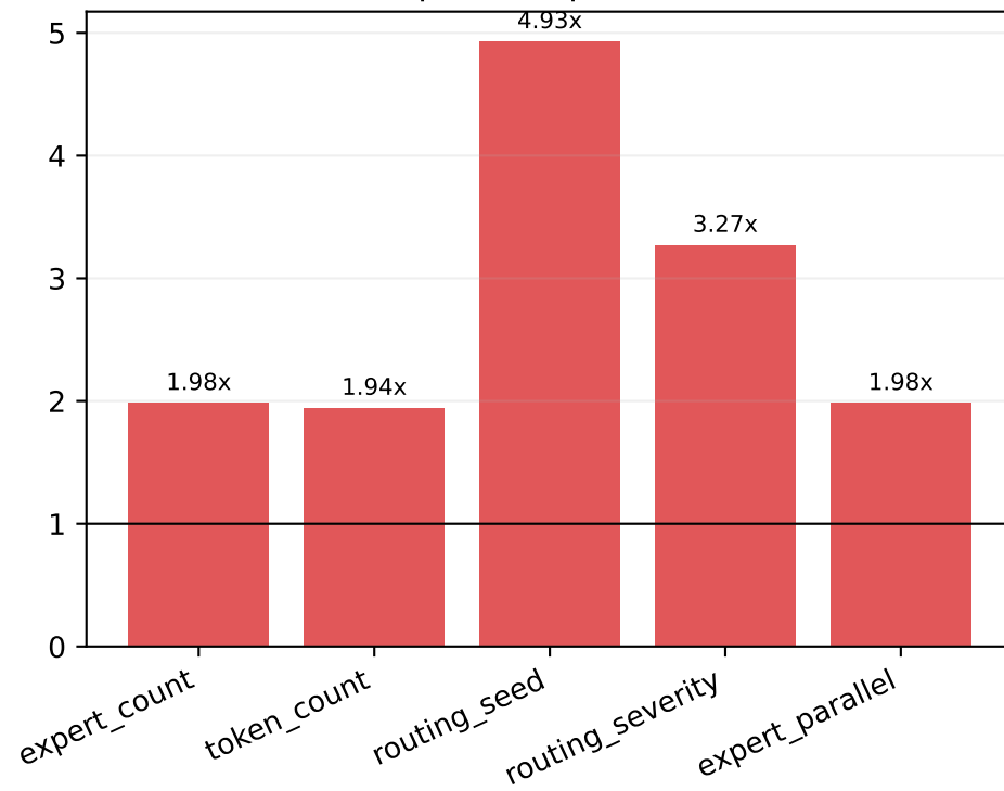
Request amplification
