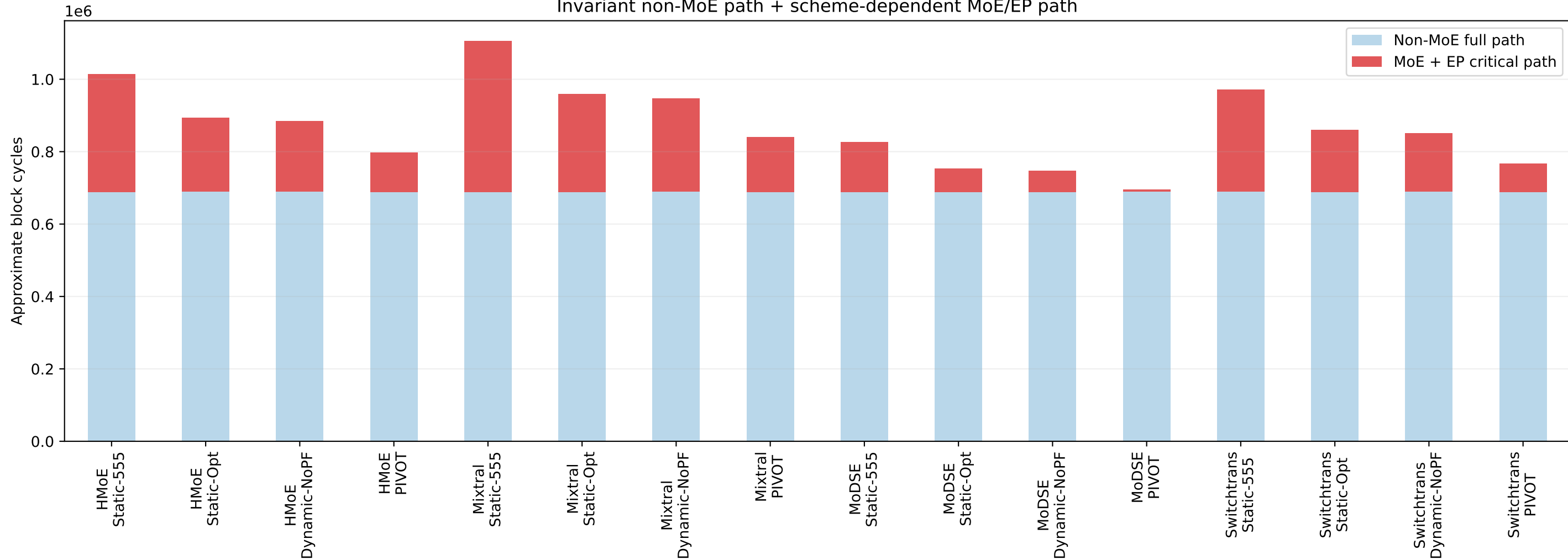
Invariant non-MoE path + scheme-dependent MoE/EP path
