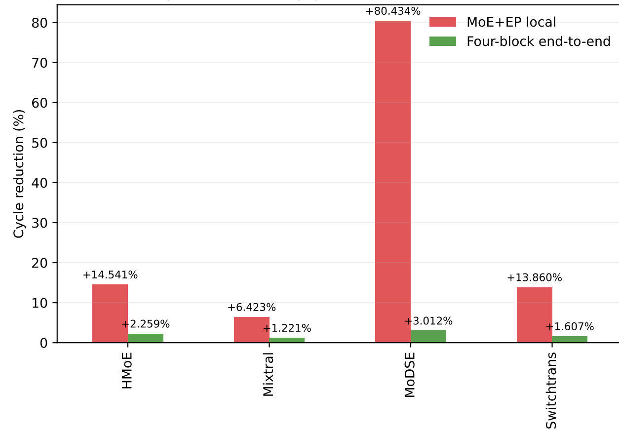
(c) Dynamic-FixedPF gap before/after Amdahl dilution
