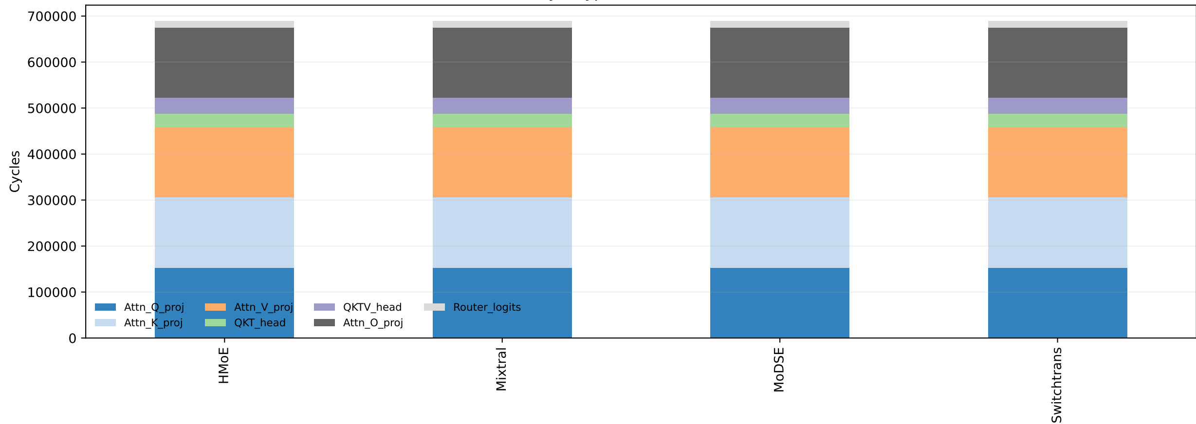
Seven non-MoE layer types accumulated across four blocks
