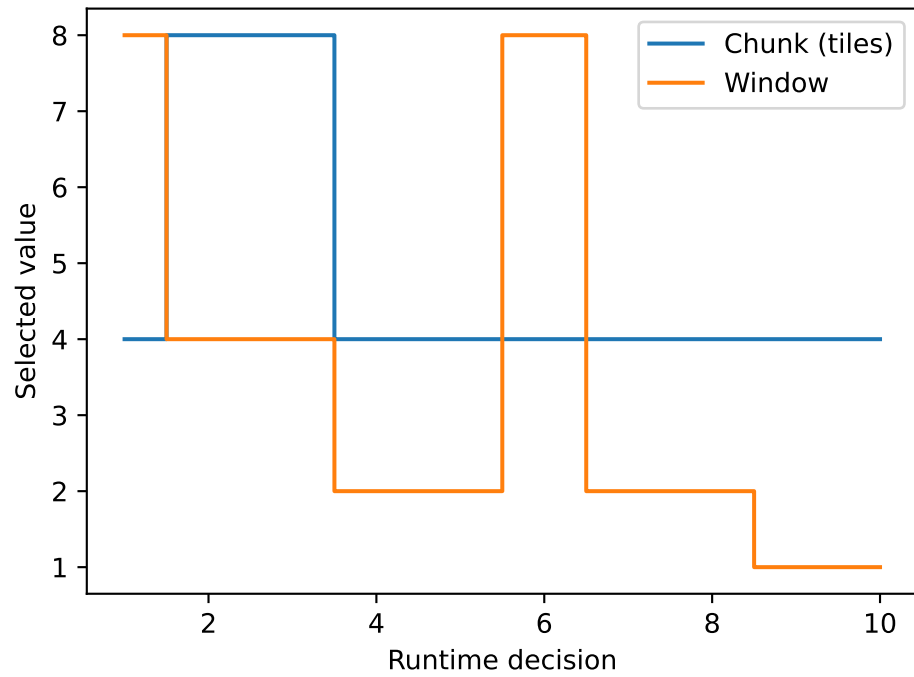
Online adaptation
