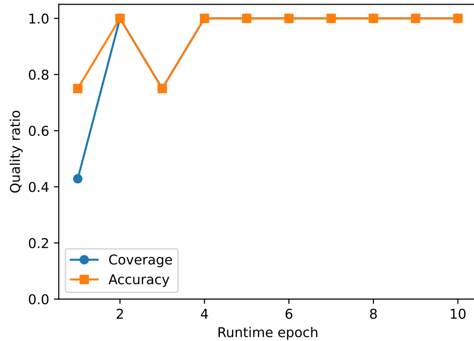
Measured quality
