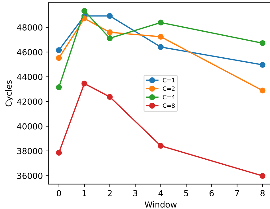
(b) Compute-transfer overlap
