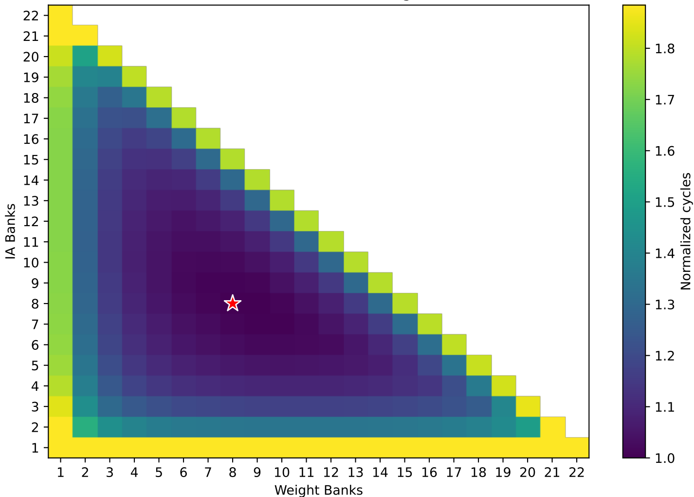
Global fixed allocation: normalized total cycles (OA Banks = 24 - IA - Weight)
