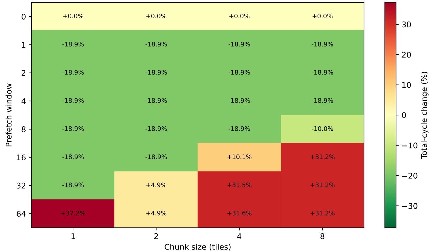
Naive prefetch total-cycle change vs NoPF (negative/green = faster; positive/red = slower)
