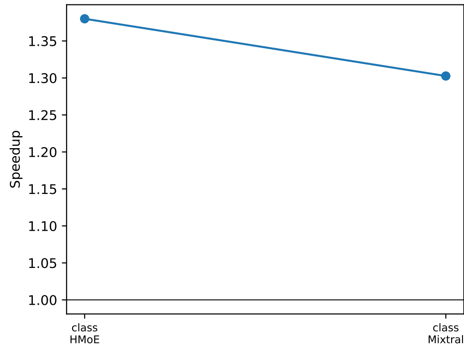
Model class
