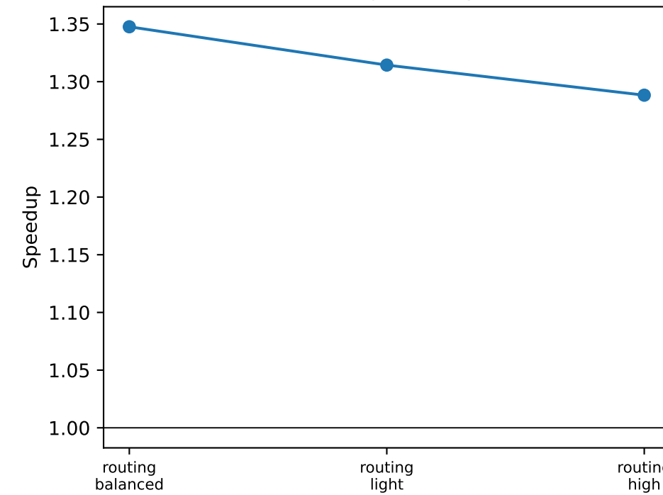
Routing severity
