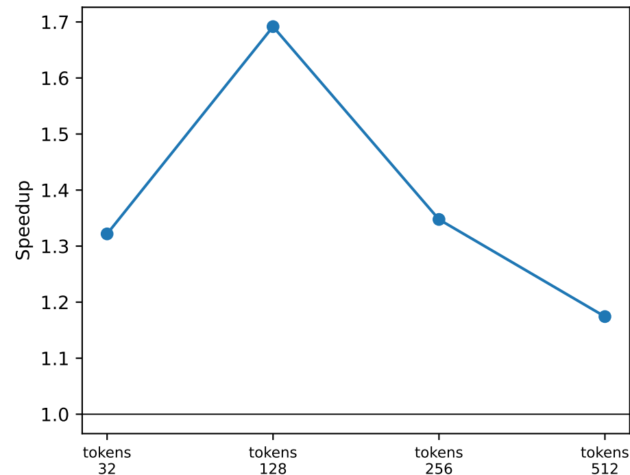
Model class
