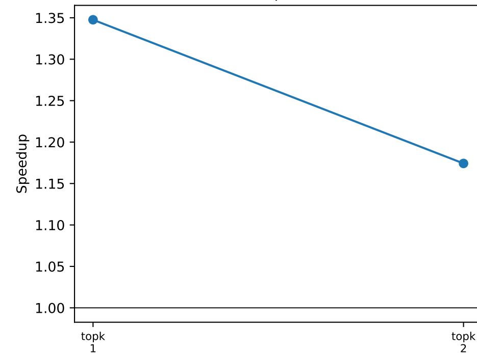
Routing severity
