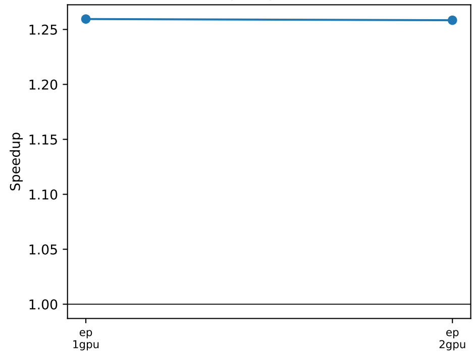
Expert parallel
