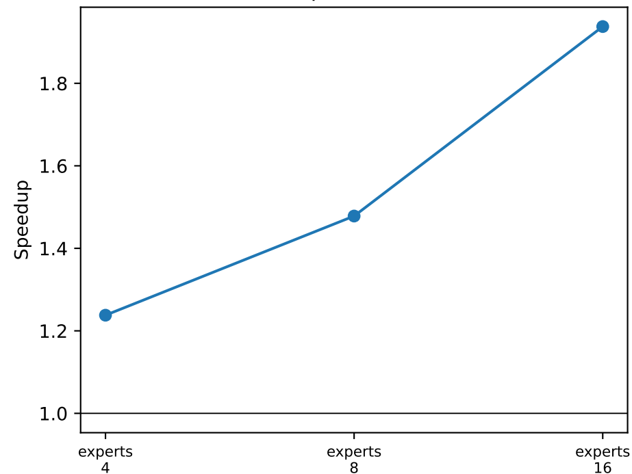
Expert parallel
