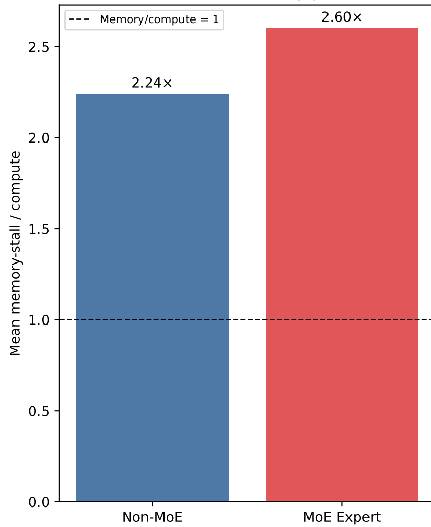
(b) Normalized memory pressure
