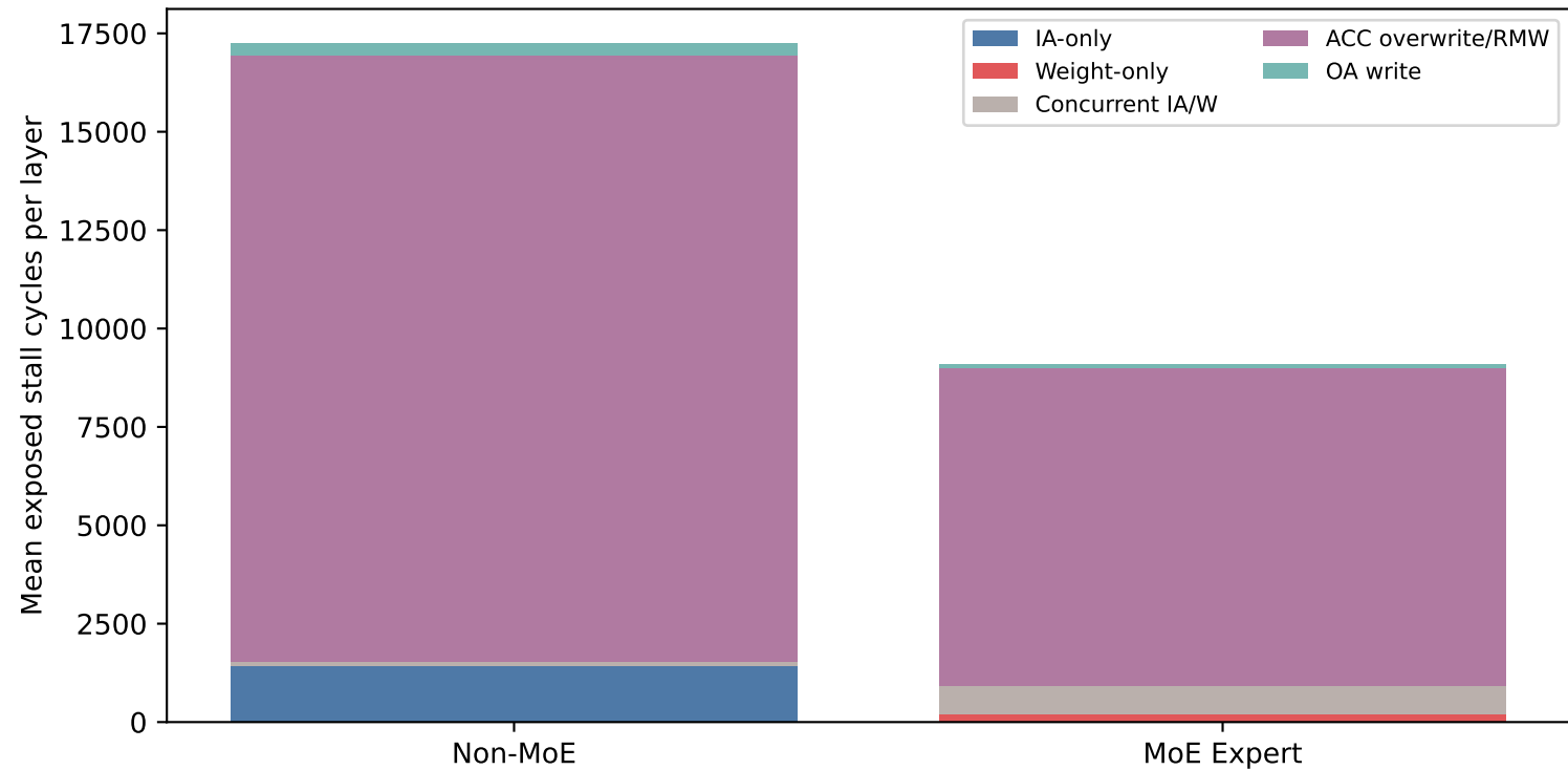
Operand and accumulator stall decomposition
