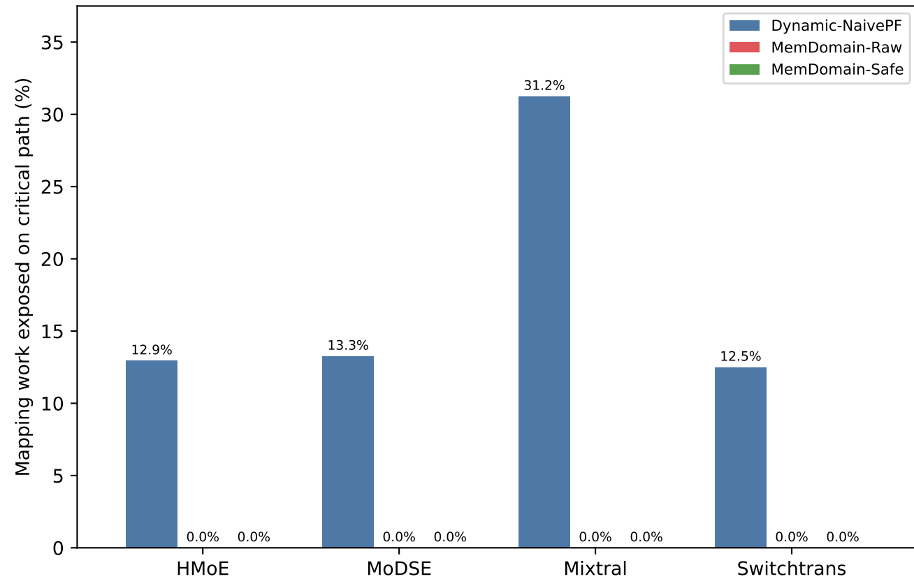
(b) How much mapping work became real overhead?
