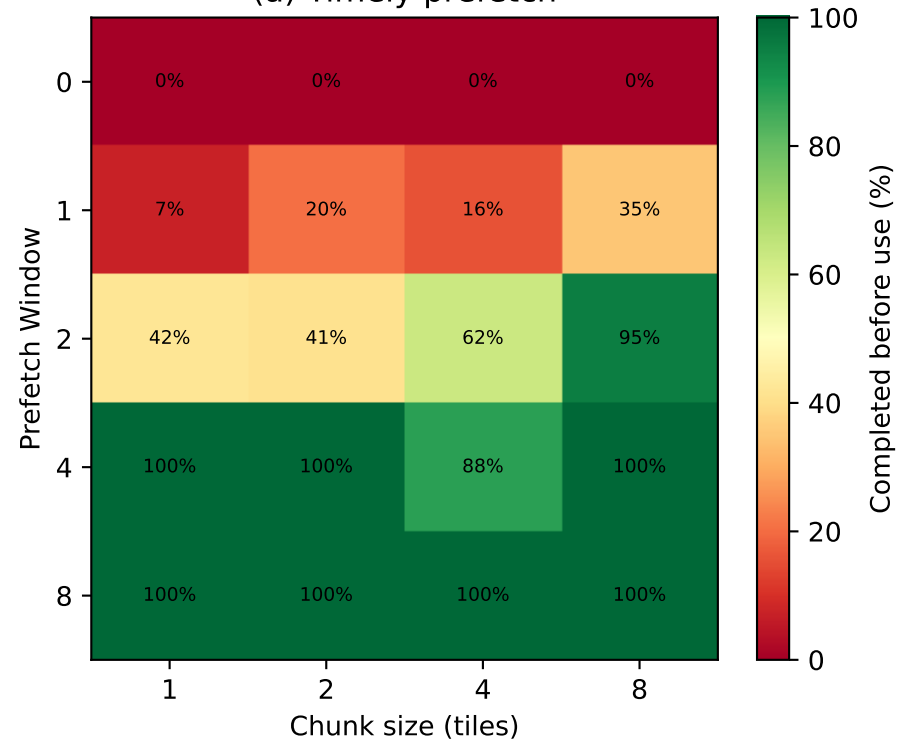
(a) Timely prefetch
