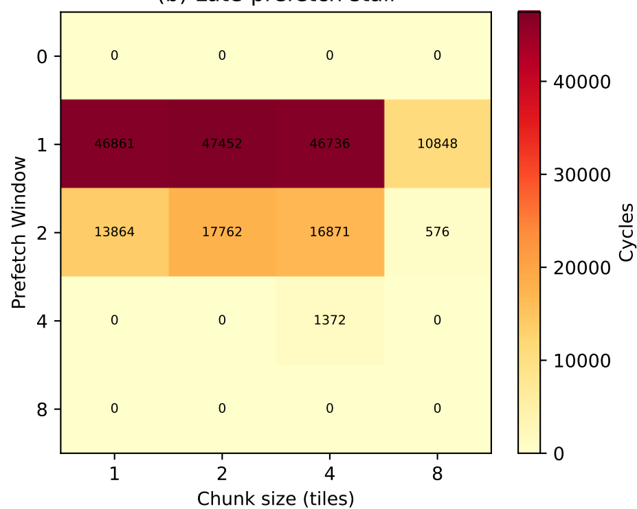
(b) Late-prefetch stall
