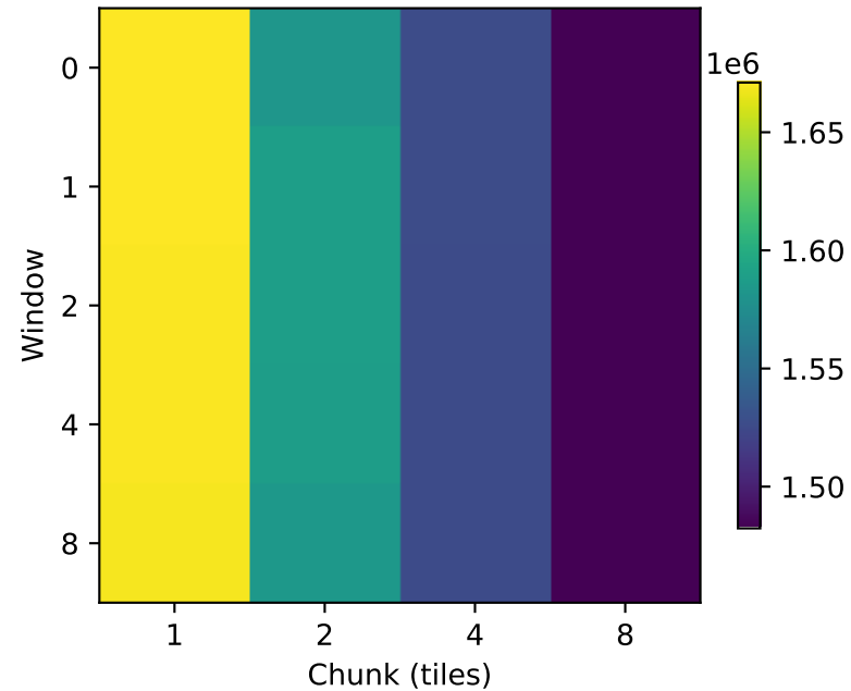
Total cycles
