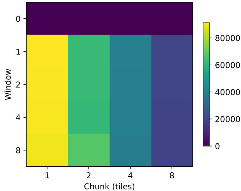
Late-prefetch stall
