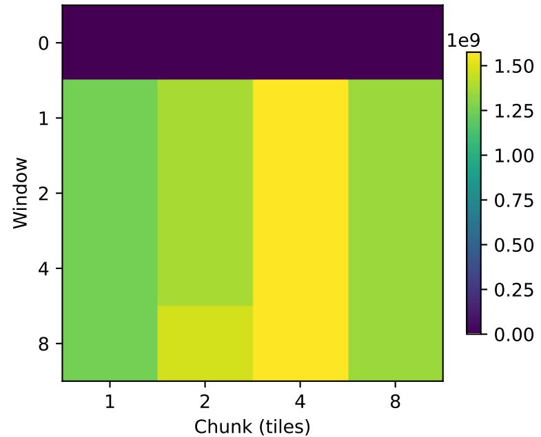
Prefetch occupancy
