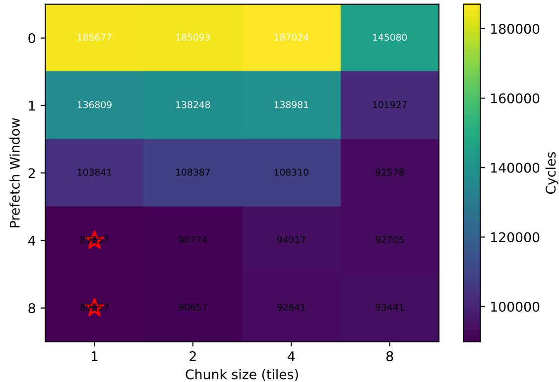
(a) Total cycles
