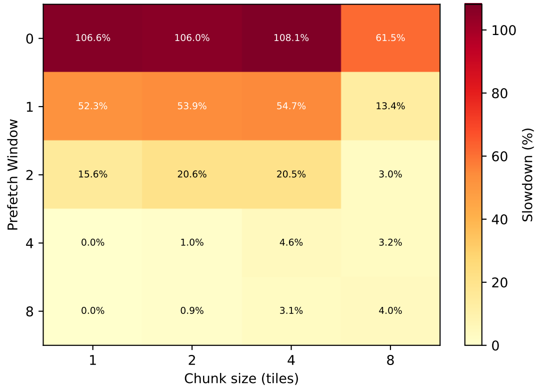
(b) Slowdown from global best
