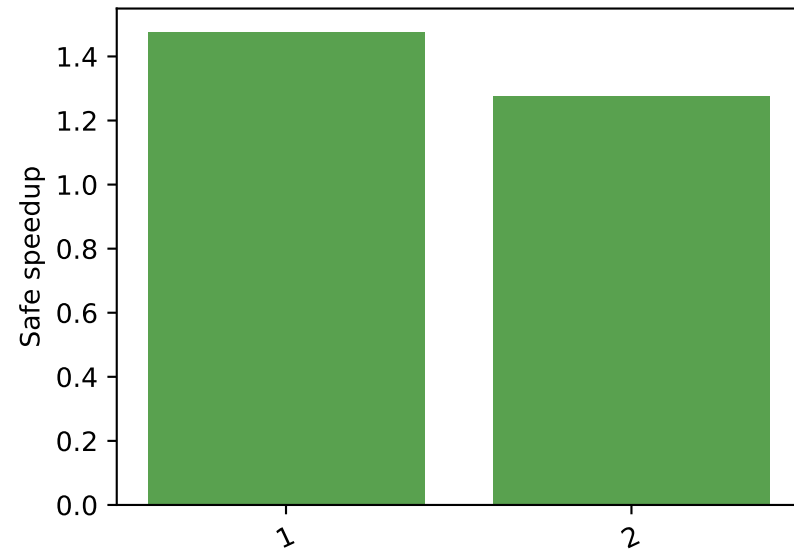
Top-K
