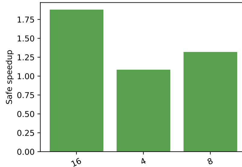
Experts
