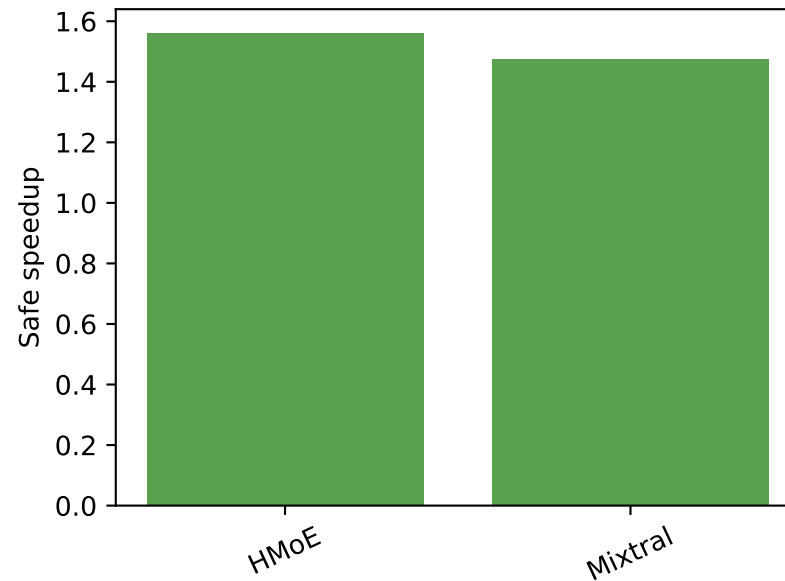
Expert sizes
