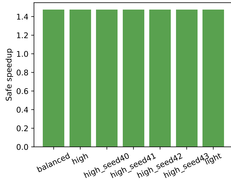
Routing
