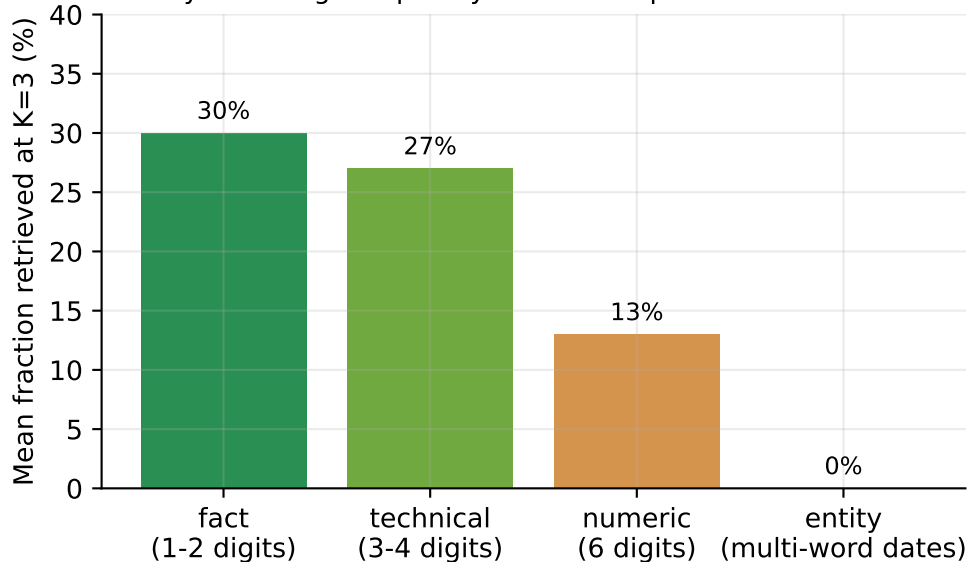
K=3 survival by decoding complexity: shorter outputs survive interference longer
