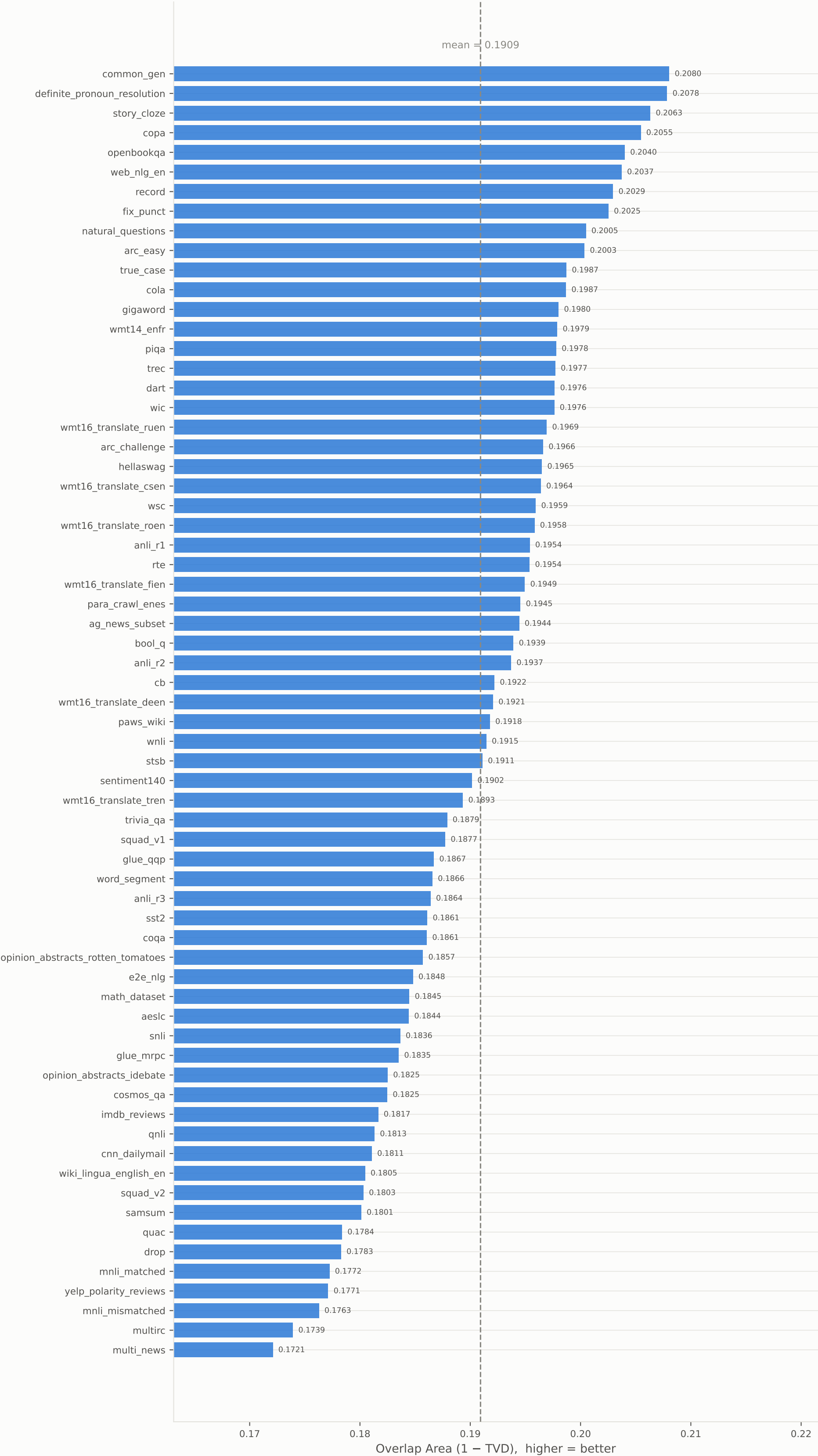
Base drafter (untrained) — Overlap Area per cluster Target: TurboSparse-Mistral-Instruct (7B) • 66 Flan clusters, model mode
