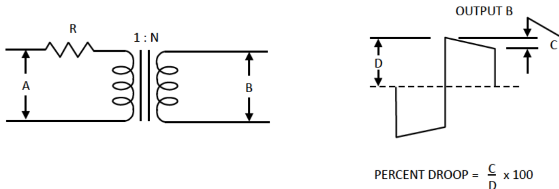
FIGURE 11. Coupling transformer.
