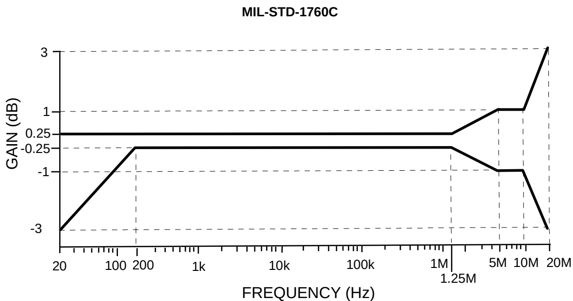
FIGURE 9. Gain misequalization envelope.
