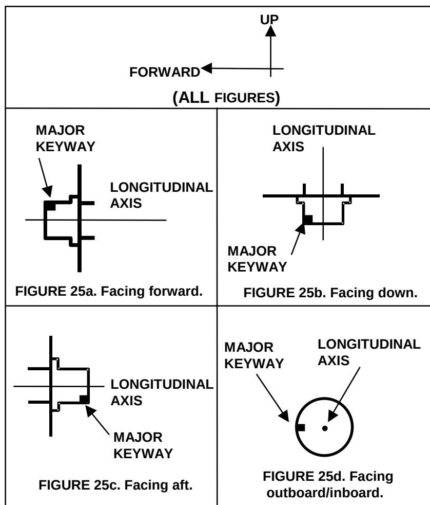
FIGURE 25. Connector orientation.
