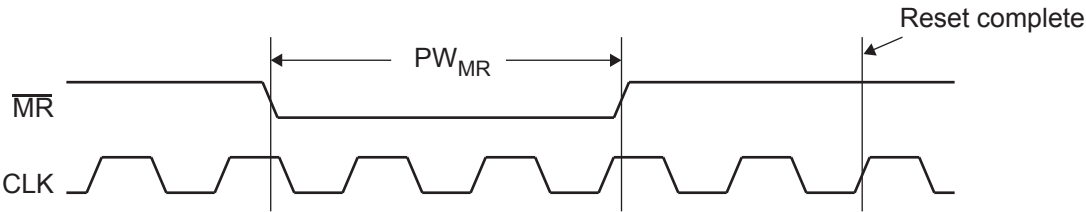
Figure 27. Master Reset Timing Diagram
