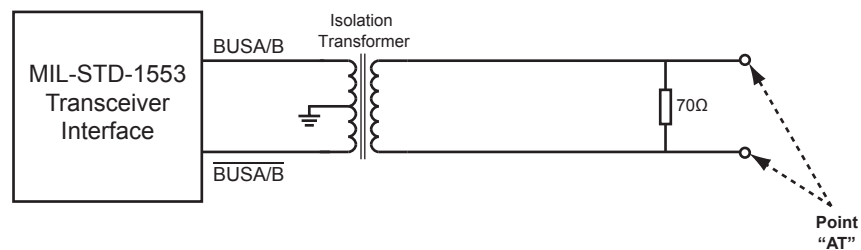
Figure 30. MIL-STD-1553 Transformer Coupled Test Circuits
