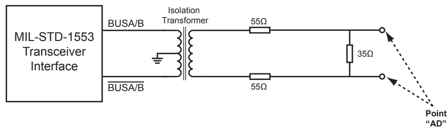
Figure 29. MIL-STD-1553 Direct Coupled Test Circuits
