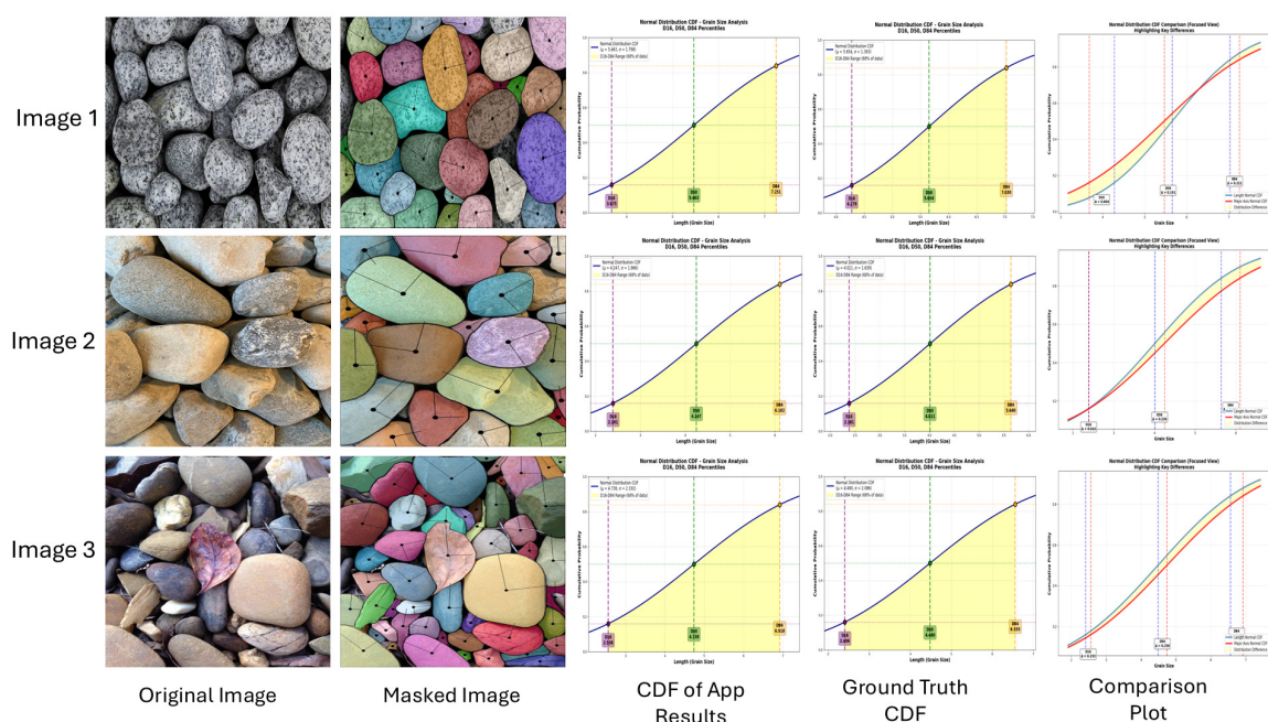
(a) Validation of mobile grain size analysis through comparison with ground truth measurements done with ImageJ across Major axes of three representative samples with D16, D50, and D84 percentiles clearly marked.
