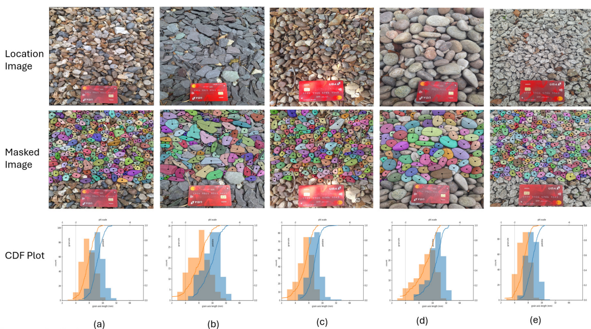
(b) Field validation of mobile grain size analysis across five diverse sediment locations (a-e) showing original images with scale cards, automated segmentation masks, and corresponding grain size distribution histograms with cumulative distribution functions for major (blue) and minor (orange) axis.
