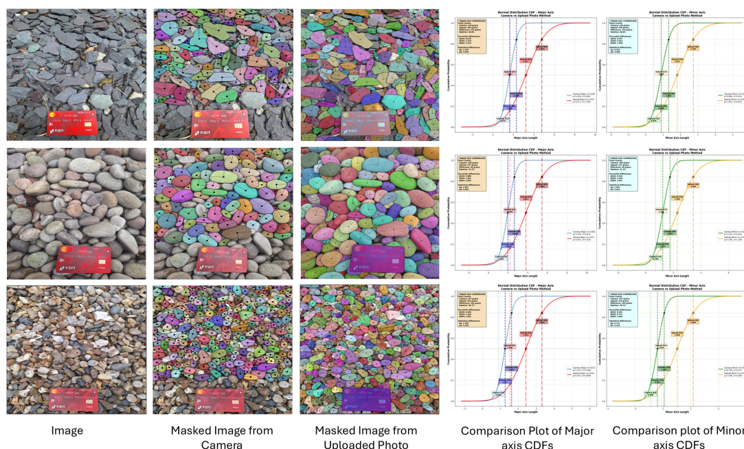
Figure 6: Comparison of camera versus upload photo methods for grain size analysis across three sediment samples, showing original images, segmentation masks, and normal distribution CDFs for major and minor axis measurements with D16, D50, D84 percentiles and grain count statistics.
