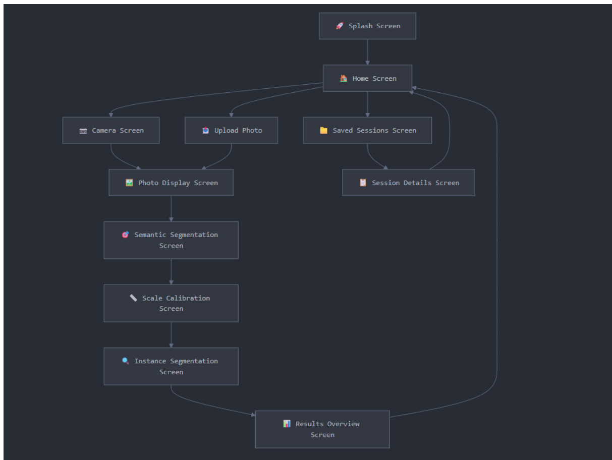
Figure 2: Navigation Flowchart of All Screens in Android Application
