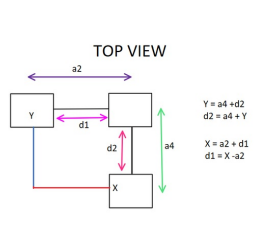
Kinematics - top
