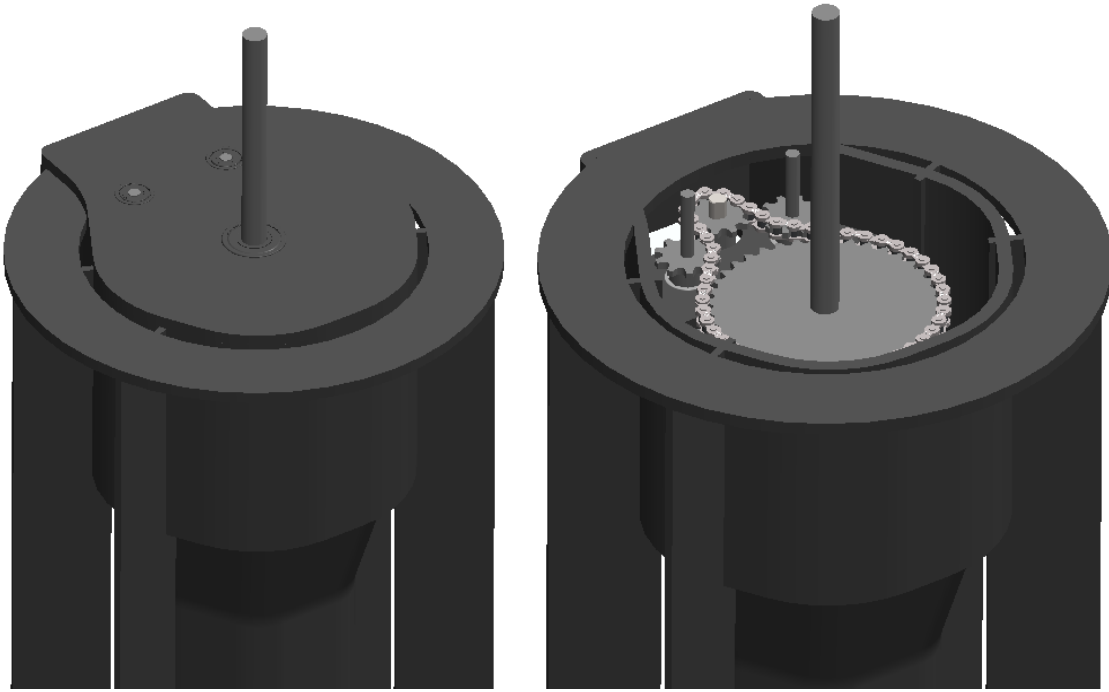
Figure 3.20 Chain and Sprocket Mechanism
