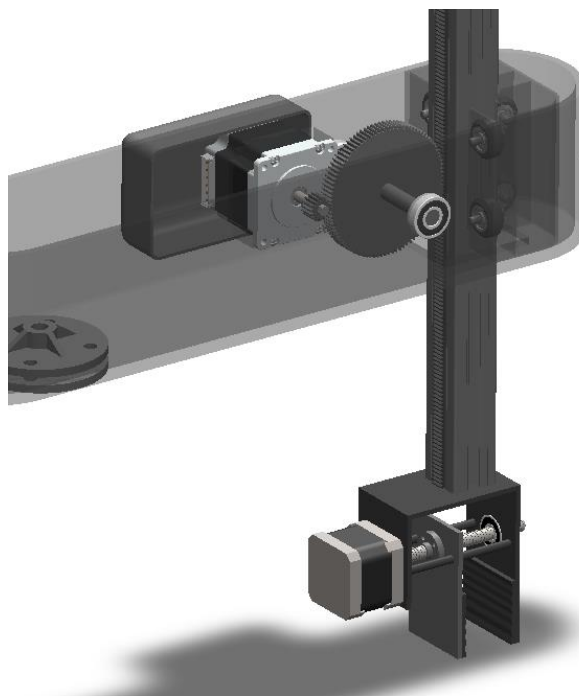
Figure 3.23 The Prismatic Joint
