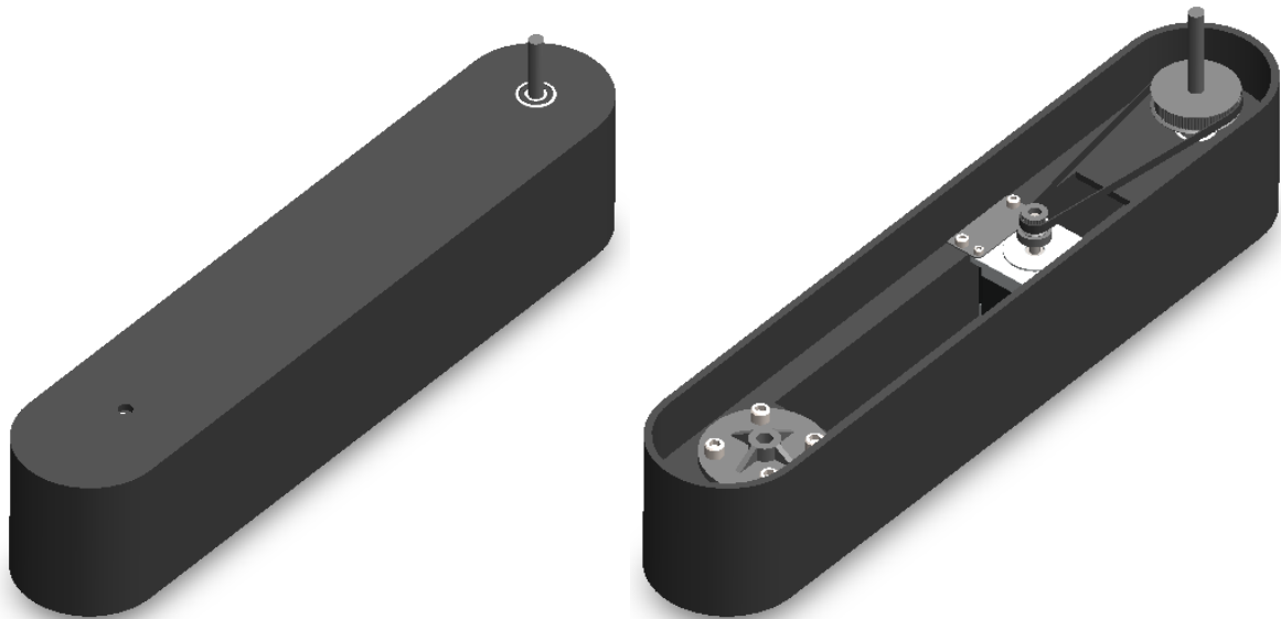
Figure 3.21 Belt and Pulley Drive Mechanism
