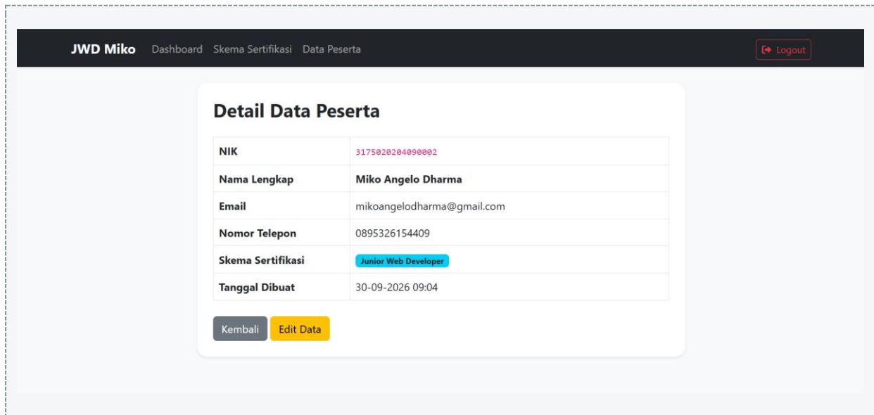
Gambar 6. Detail Peserta
