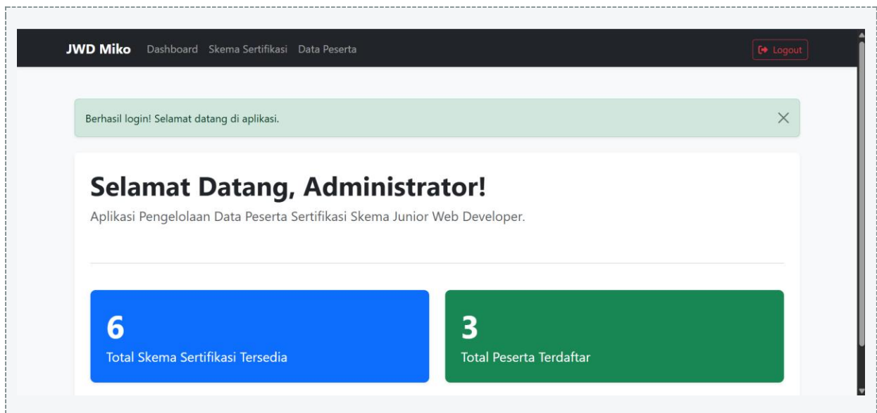
Gambar 3. Dashboard
