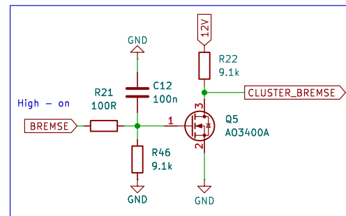
BREAKS ERROR control
