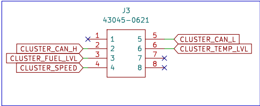
Cluster data lines
