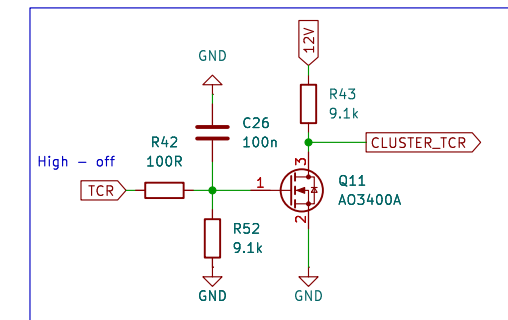
COOLANT ERROR control
