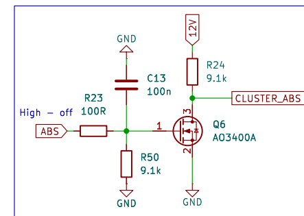
ABS ERROR control
