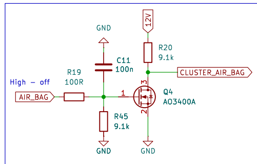
AIR BAG control
