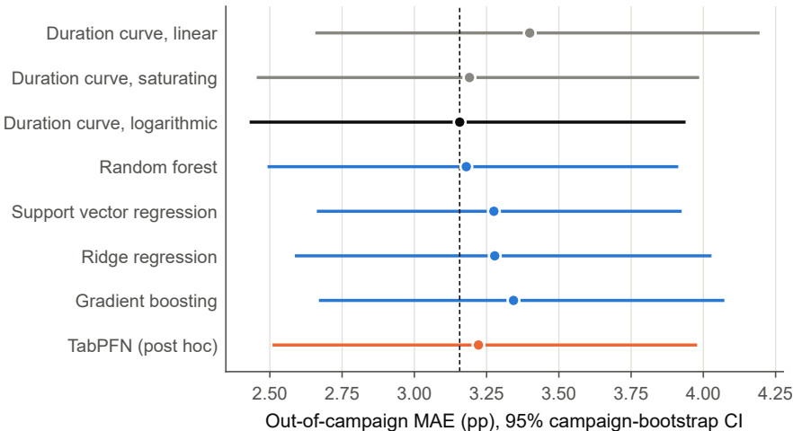
a Error in held-out campaigns
