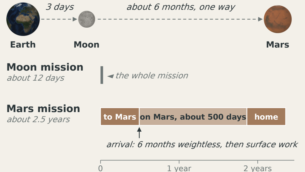
Figure 2. Moon mission vs Mars mission
