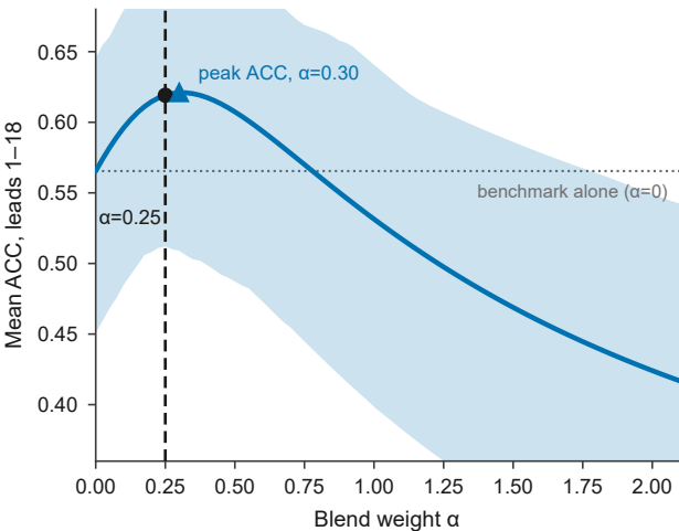
(a) \alpha = 0.25 sits close to the ACC optimum
