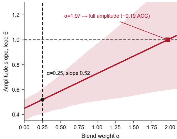
(b) Full amplitude is available — at a cost in skill
