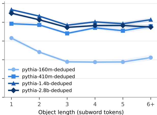
(b) In-context control (answer given)
