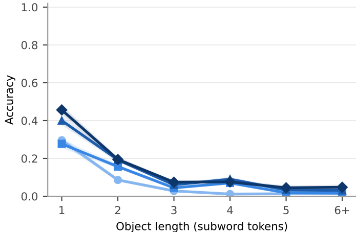
(a) Factual recall
