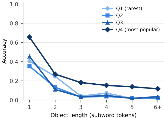
Within subject-popularity quartiles (pythia-2.8b-deduped)
