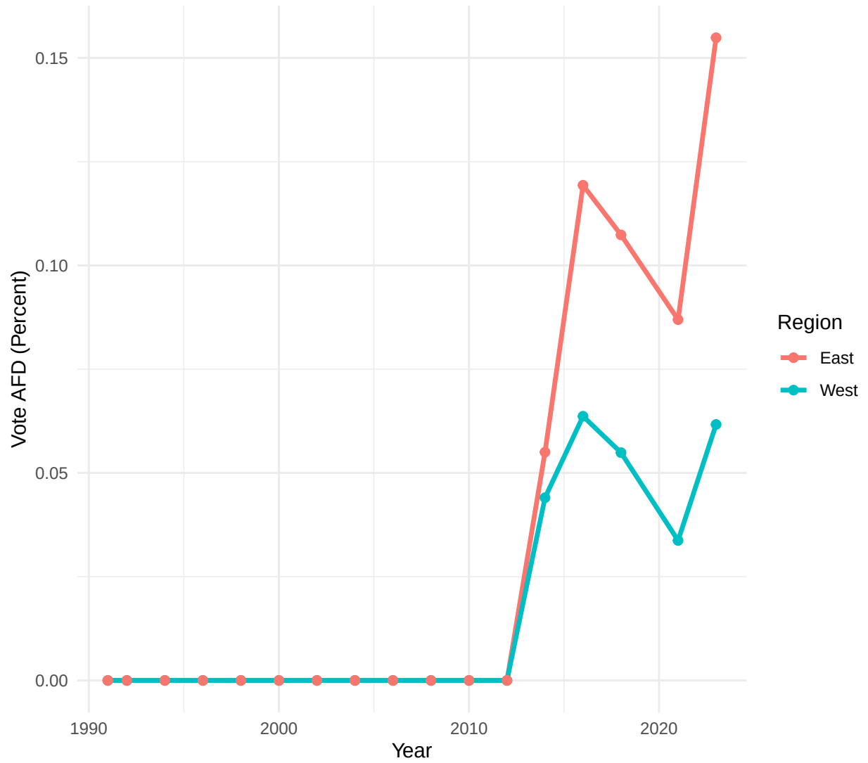
Development of willingness to vote AFD
