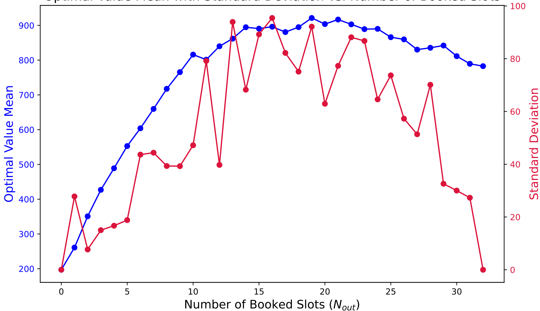
Optimal Value Mean with Standard Deviation vs. Number of Booked Slots
