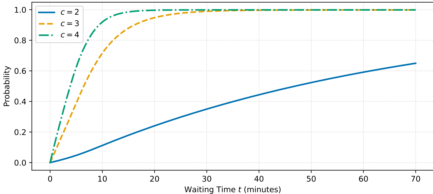
M/G/c Conditional Waiting Time Distribution
