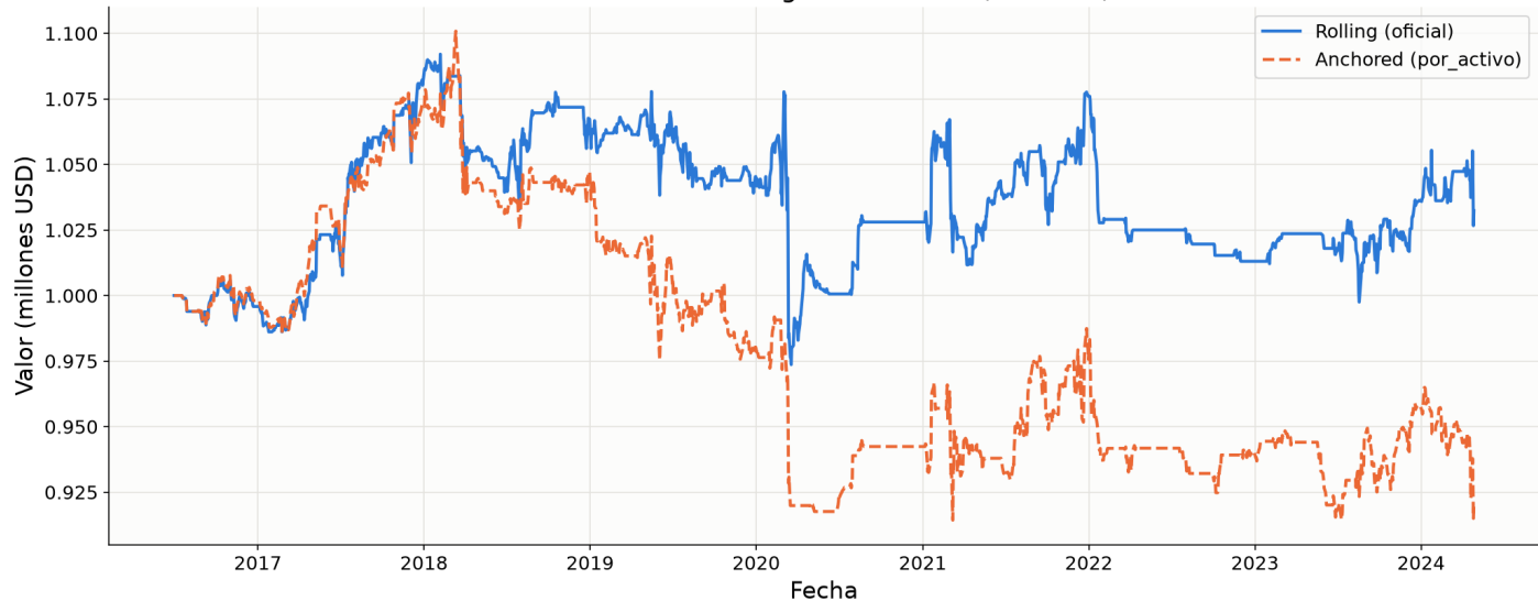
Walk-forward rolling vs. anchored (WF-OOS)
