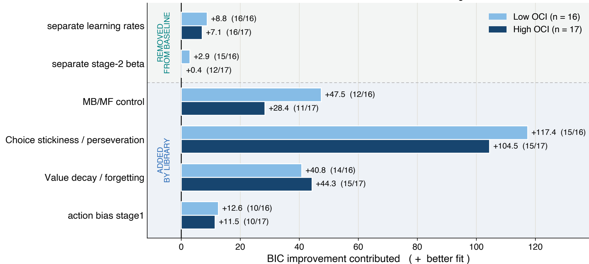
Mechanisms most different between Low and High OCI
