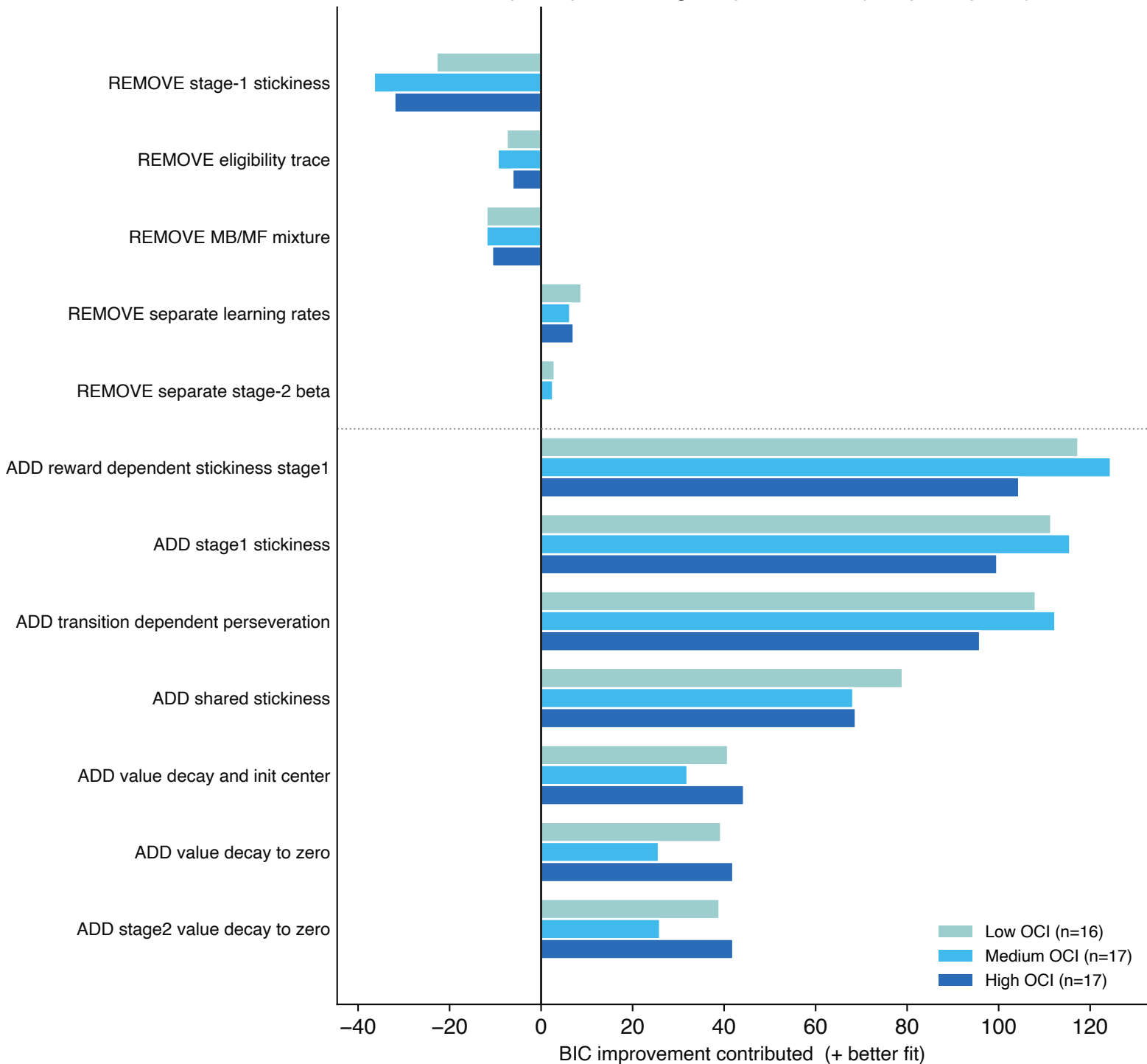
Library component ledger, by OCI tertile (test participants)
