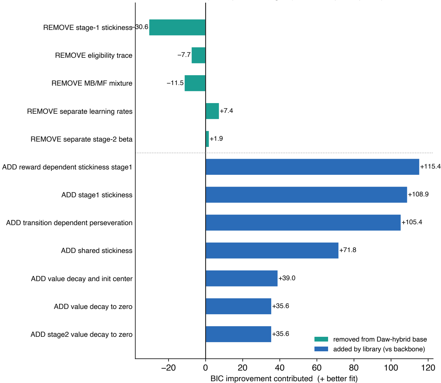
Library component ledger (all 50 test participants)
