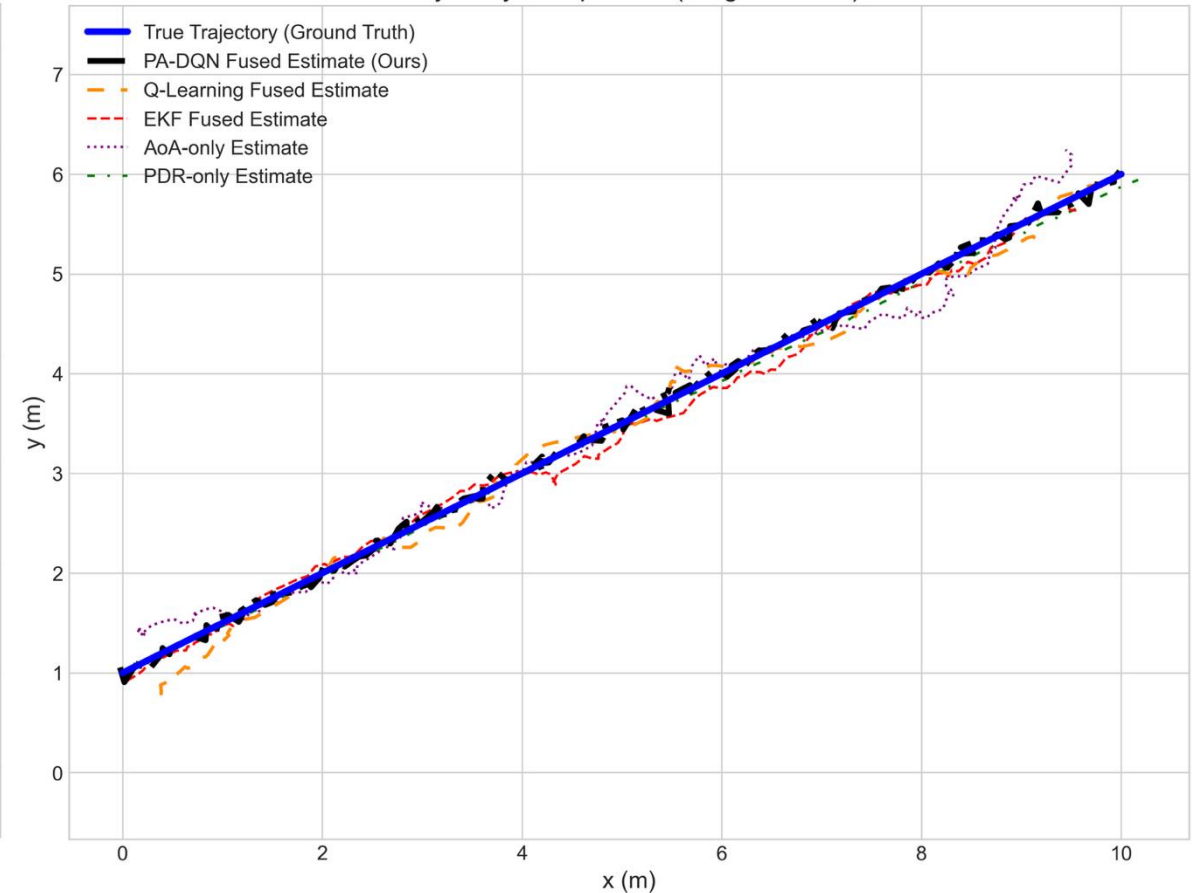
Trajectory Comparison (Diagonal Path)
