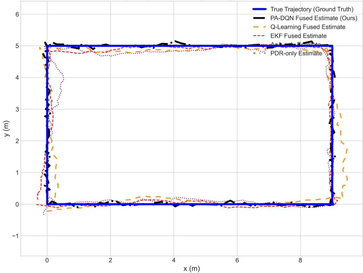
Trajectory Comparison (Rectangular Path)
