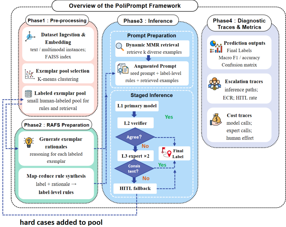
Figure 1: Overview of the PoliPrompt framework. Phase 1 constructs a labeled exemplar pool from the input data. Phase 2 generates exemplar rationales and synthesizes label-level rules through RAFS. Phase 3 assembles query-time augmented prompts through dynamic retrieval and performs staged inference with expert escalation and HITL fallback. The framework produces final labels together with diagnostic traces, including ECR, HITL rate, inference paths, and cost signals.
