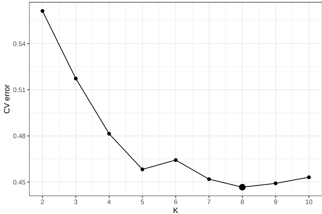
ADMIXTURE cross-validation error, best K = 8
