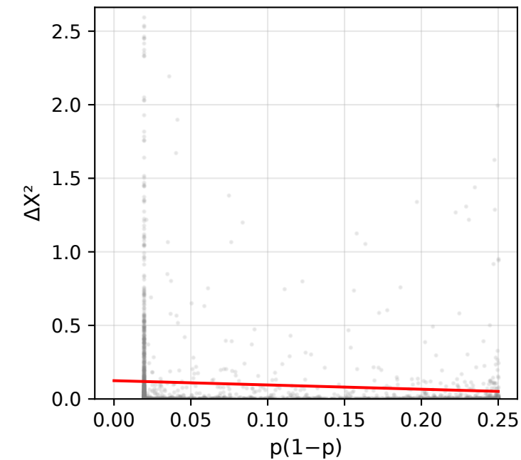
4. Boundary scaling (slope=-0.291)
